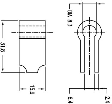
BOLT RETAINER
