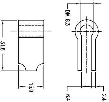
BOLT RETAINER
